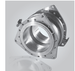
Fig. 8.3 Chamber expansion joint made of titanium for the chemical industry
