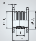
Type ABN with inner sleeve
