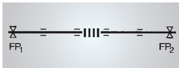
Fig. 9.6 Symmetrical arrangement of the expansion joint. Frictional force distributed uniformly.
