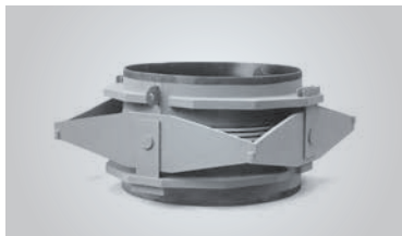
Fig. 3.15 Gimbal expansion joint "WRK"
