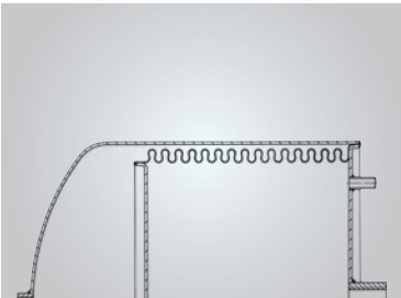
Fig. 8.33 Volumetric compensation container
