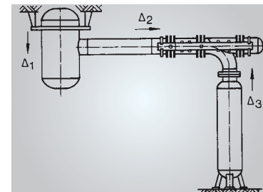
Fig. 12.16 Elbow-connected pressure balanced lateral expansion joint
