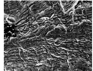
Fig. 2.9 Fatigue fracture under the scanning electron microscope
