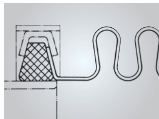
Fig. 7.4 moVix connection
