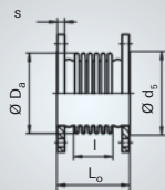
Type ABN without inner sleeve
