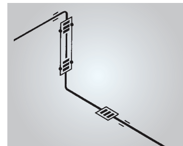
Fig. 9.28 3-dimensional three-hinge system with lateral and angular expansion joints
