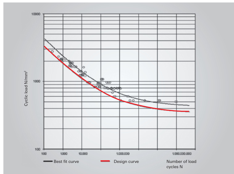
Fig. 11.2 Determining the S-N curve
